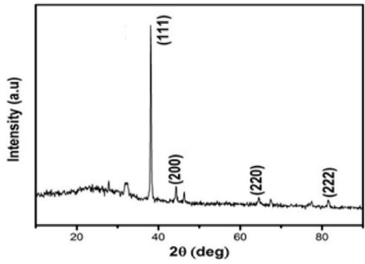
Figure 4. XRD pattern of synthesized AgNP's using Leptogium marginellum extract
