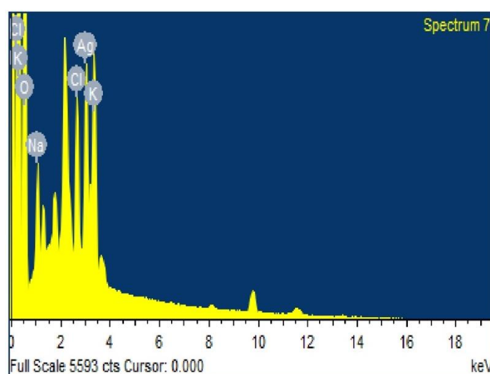
Figure 3. EDX spectroscopy unveiling the chemical components of the synthesized AgNP's using Leptogium marginellum extract
