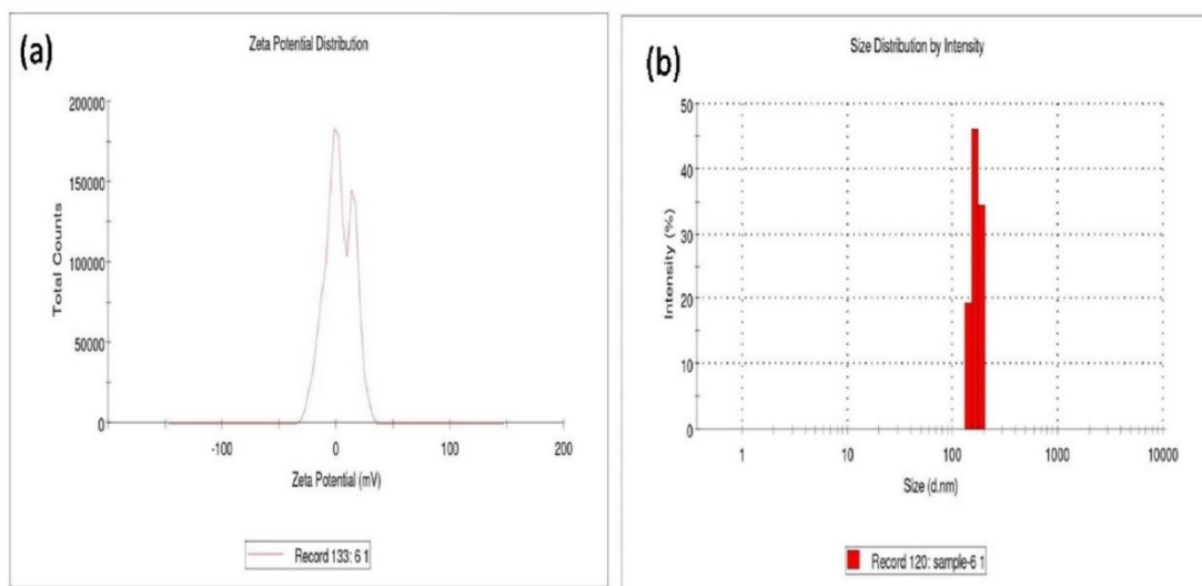
Figure 5 (a, b). Zeta potential and hydrodynamic diameter of AgNP's using Leptogium marginellum extract
